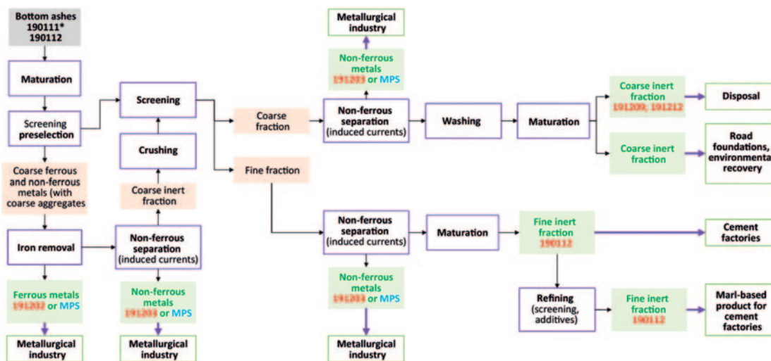
Figure 4.4 - Example of heavy ash treatment plant
