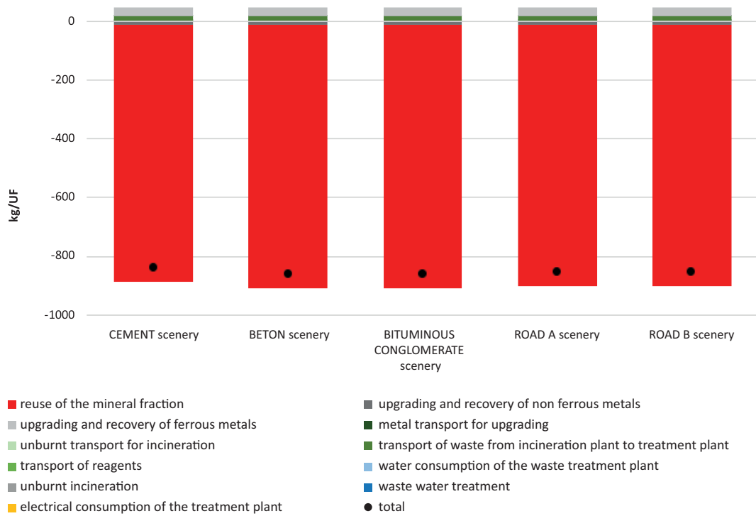
Figure 4.5 - Indicator of natural mineral resource consumption associated with the treatment of 1 tonne of heavy ash and recovering the metals contained therein and the resulting mineral fraction, for five different alternatives of using the latter
