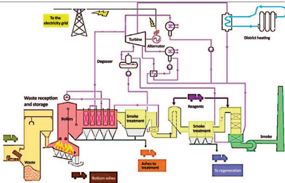
Figure 2.3 - Incineration plant diagram (TRM, 2019)
