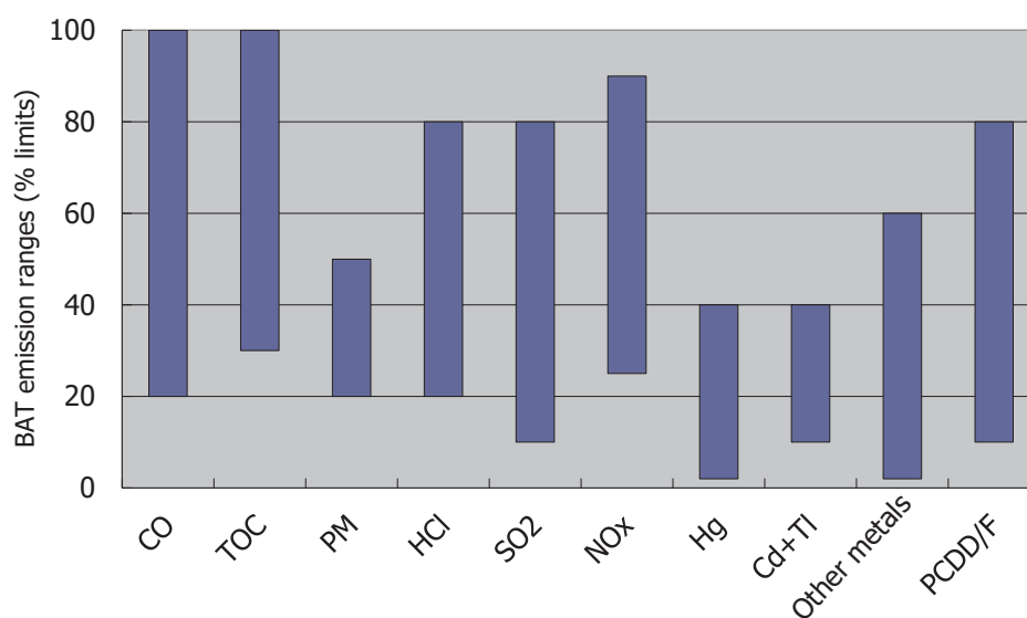
Figure 3.1 - Comparison of emission limits for European installations and ranges associated with sector BAT
