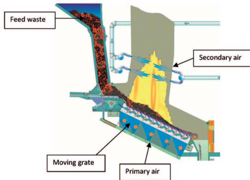
Figure 2.4 - Functional diagram of the moving grille furnace (Bourtsalas, 2020)
