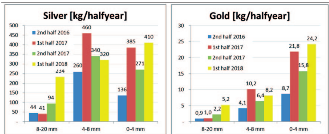
Figure 4.3 - Quantities of silver and gold recovered from heavy ash at a treatment plant in the Netherlands (Born, 2018). It is noted, in particular for gold, the significant presence in the fraction less than 4 mm
