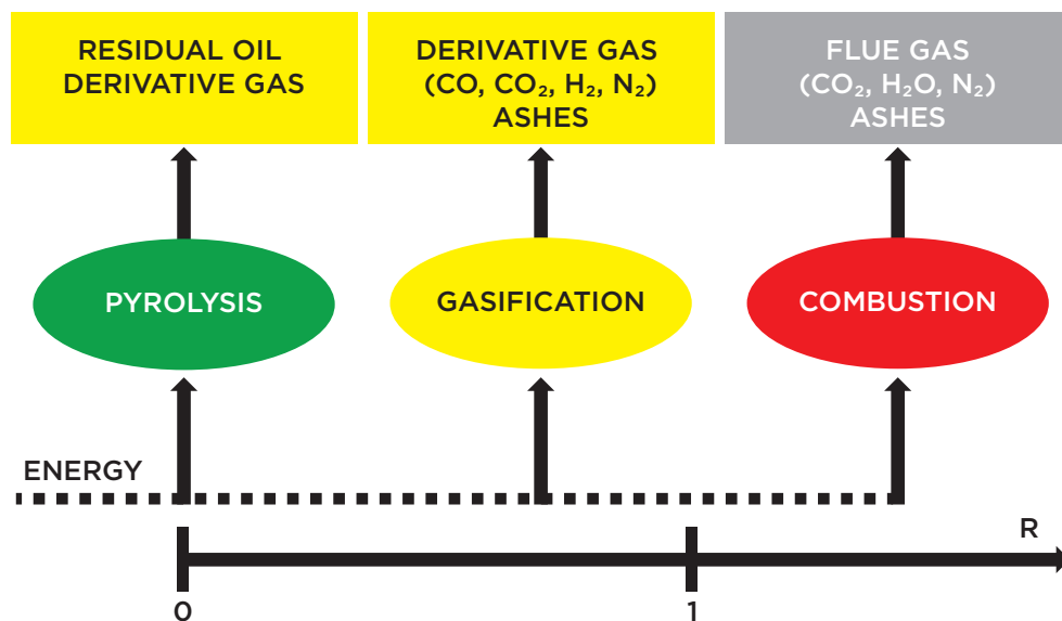
Figure 2.2 - Schematic representation of heat treatment processes (ENEA, 2008)
