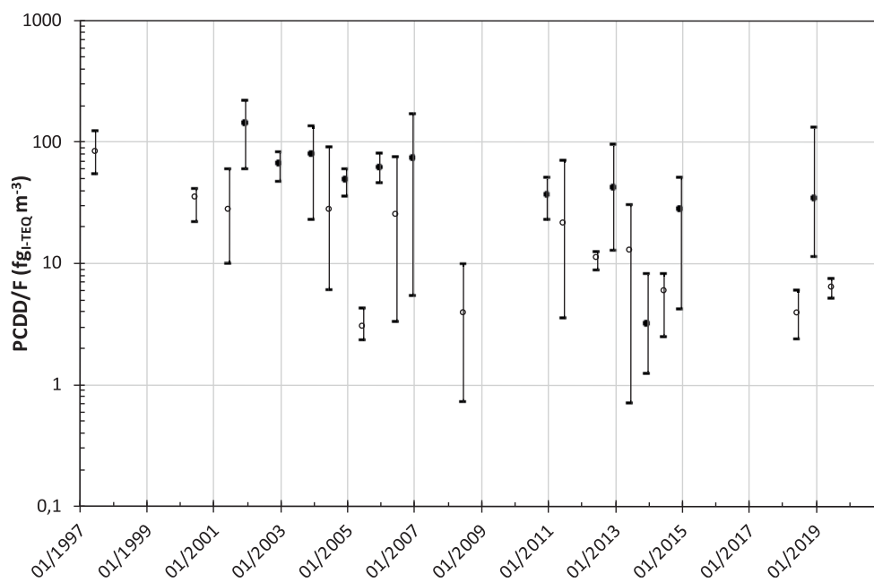
Figure 3.3 - Seasonal concentrations (mean, minimum and maximum weekly samples) of dioxins detected in different monitoring sites in the area of incineration plant location in the Po Valley (empty indicators: summer season; full indicators: winter season)
