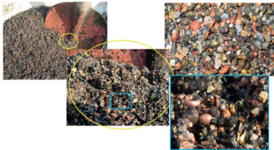
Figure 4.2 - Heavy non-ferrous metal component recovered from dry extracted incineration bottom ash. In particular, the presence of copper is evident
