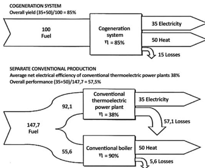
Figure 2.5 - Comparison between combined and separate production of the same quantities of electricity and heat
