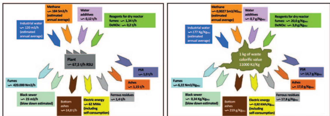
Figure 2.6 - Hourly mass balance and balance for 1 kg of waste treated by the Turin incineration plant
