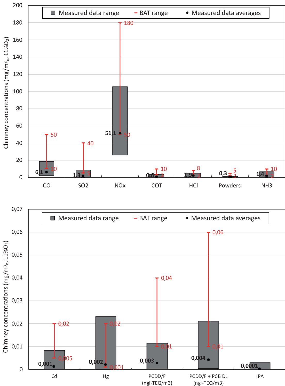
Figure 3.2 - Comparison of emission measurements measured in the three-year period 2016-2018 by Italian plants and ranges associated with industry BAT for conventional (a) and trace toxic contaminants (b).
