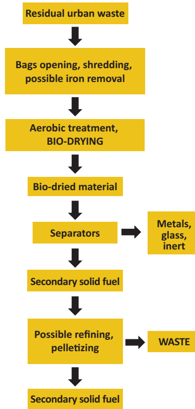
Figure 5.2 - Diagram of an MBT with biostabilisation process
