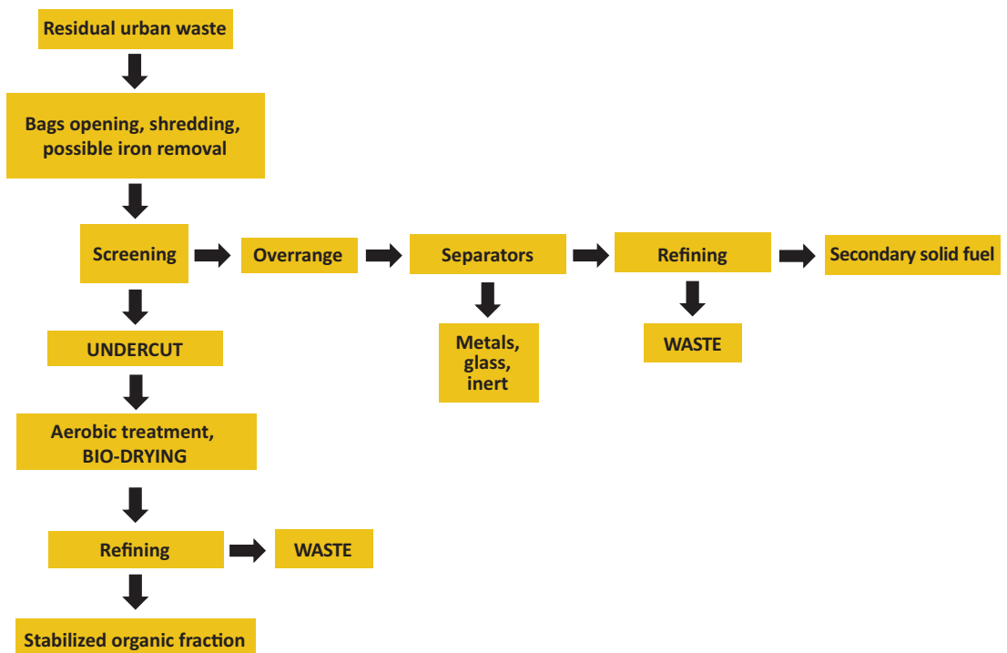
Figure 5.2 - Diagram of an MBT with biostabilisation process
