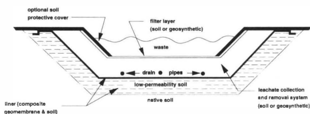
FIG. 2 GENERIC LINER DESIGN FOR NONHAZARDOUS WASTE FACILITY.
