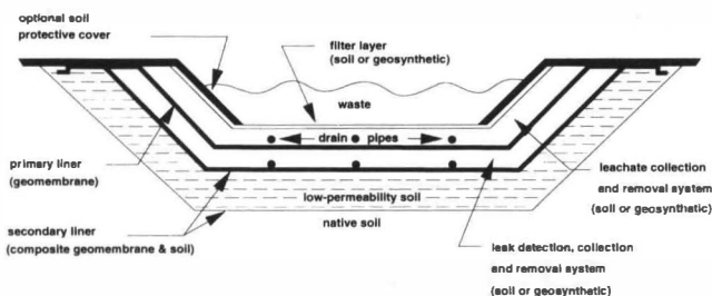
FIG. 1 SCHEMATIC OF DOUBLE LINER SYSTEM.
