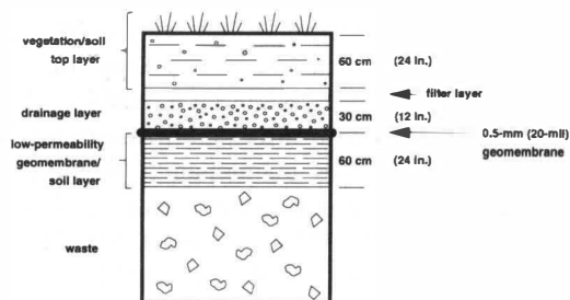
FIG. 3 USEPA-RECOMMENDED LANDFILL COVER DESIGN.
